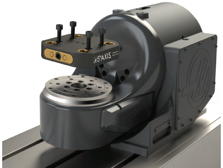
Haas TRT160 configuration
